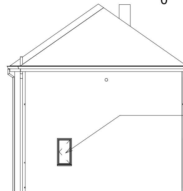
4 West elevation 1 : 100
